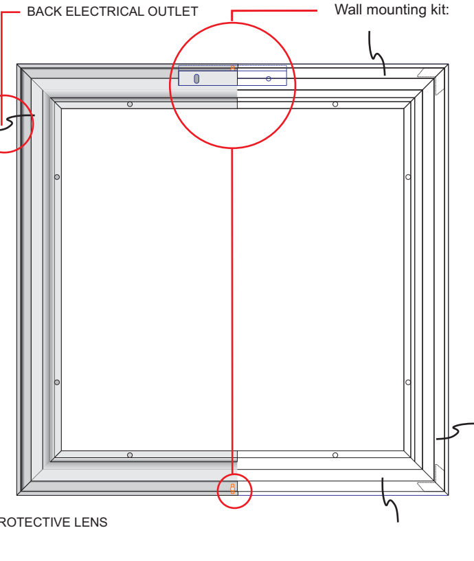
BACK VIEW
