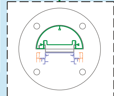
PHP7500 Post D: 7" [178 mm]
