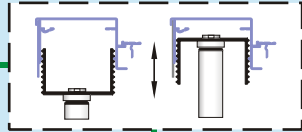
PHP4009 Adjustable raceway cover D: 1" [25 mm] W: 1 3/4" [44 mm]
