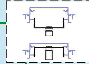
UN5579 Adjustable raceway cover D: 1" [25 mm] W: 3 1/2" [89 mm]
